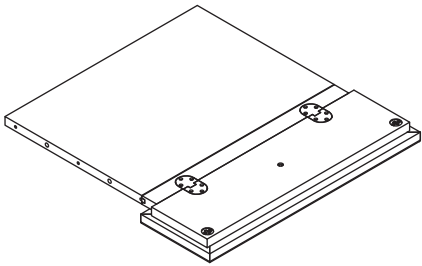
(15) AVANTTIROIR (2 PCS)
